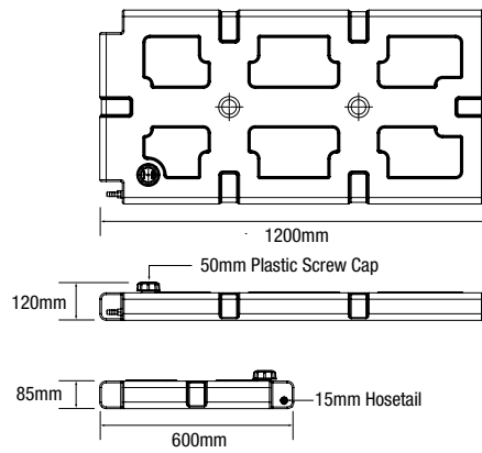
IWT004 - 50L ROOF RACK TANK
