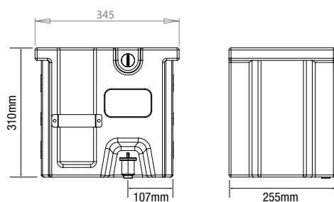
IWT008 - 15L UNDER TRAY HAND WASH TANK
